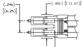
LC UNIBODY DUPLEX CONNECTOR ASSEMBLIES WITH UNJACKETED CABLE BOOT
