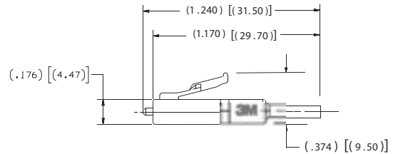
LC BTW CONNECTOR (BEHIND THE WALL) UNJACKETED FIBER AND SIMPLEX ONLY
