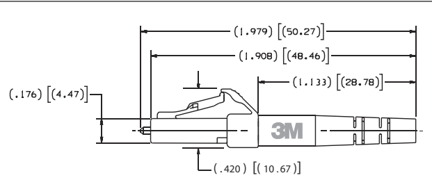
LC UNIBODY DUPLEX CONNECTOR ASSEMBLIES WITH JACKETED CABLE BOOT
